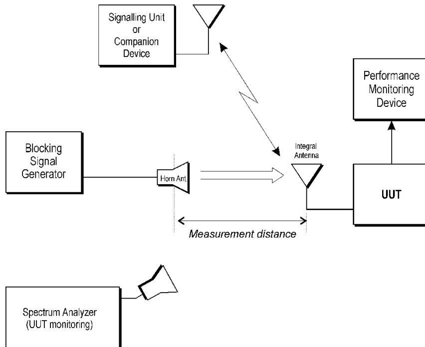
Figure C.4: Measurement Set-up
